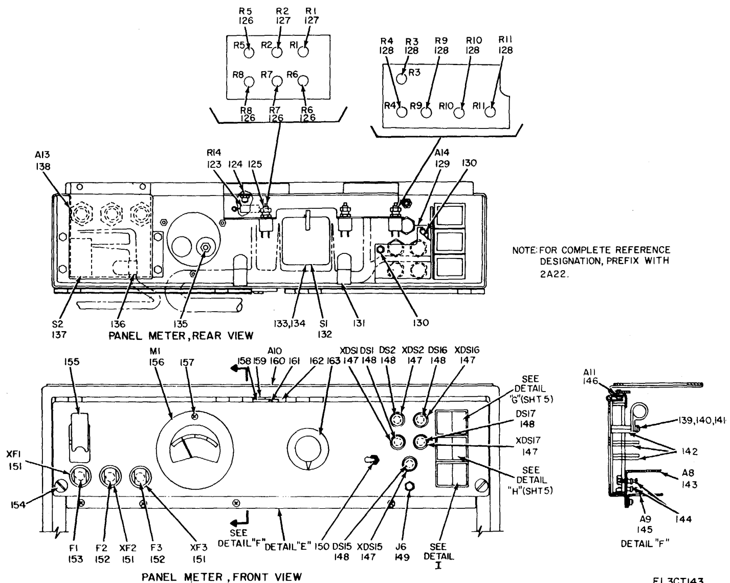
Figure 36. Cabinet, Electrical Equipment 2A22 (3 of 4).
