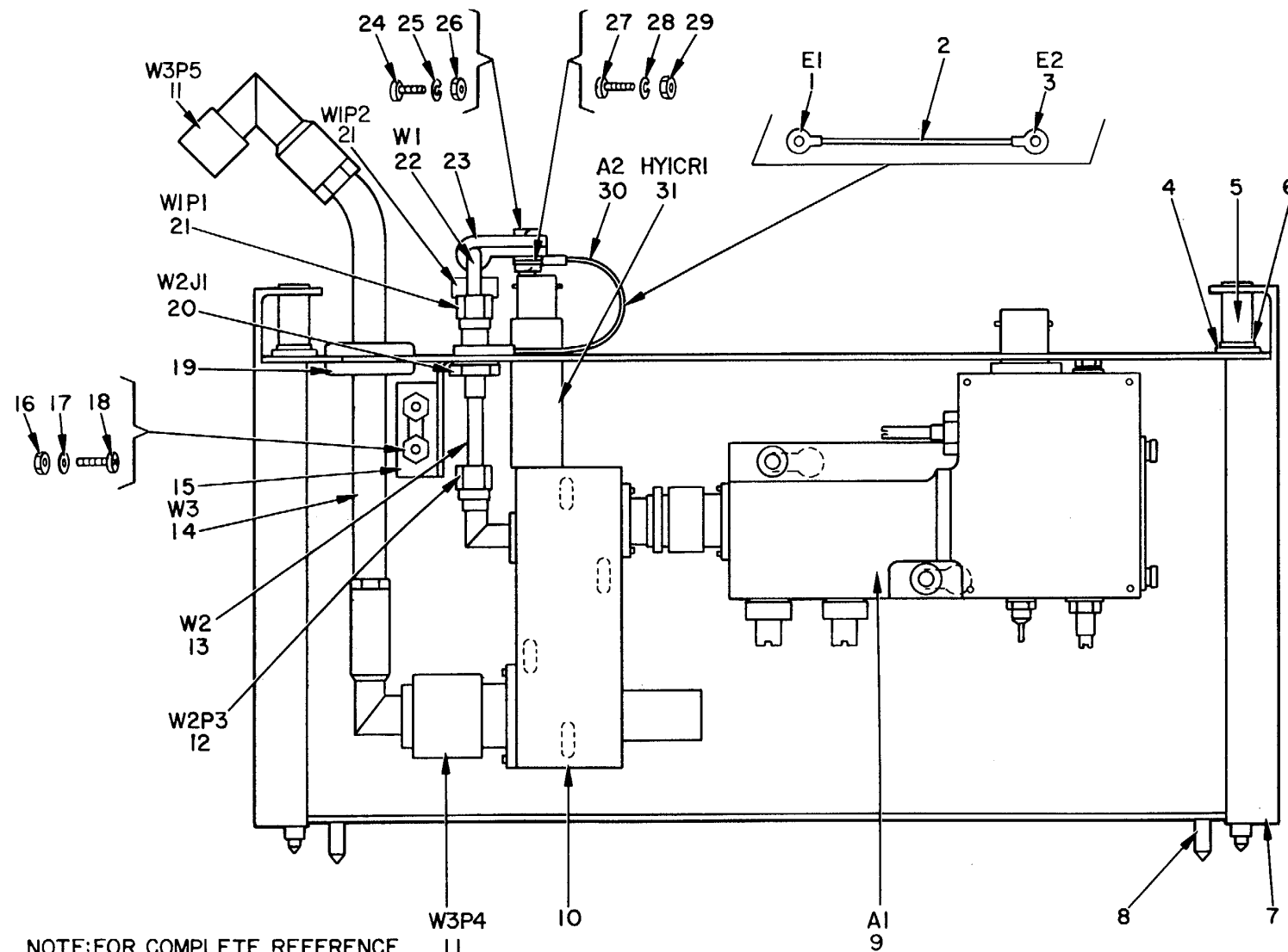
Figure 8. Mixer Stage, Frequency Transmitter 1A9.
