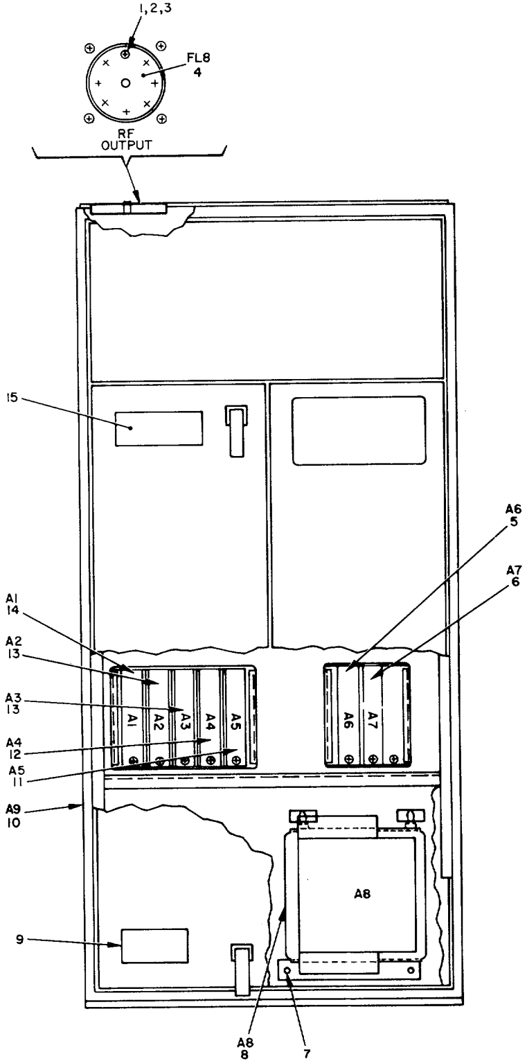
Figure 38. Amplifier, Radio Frequency AM-6090/GRC-143.
