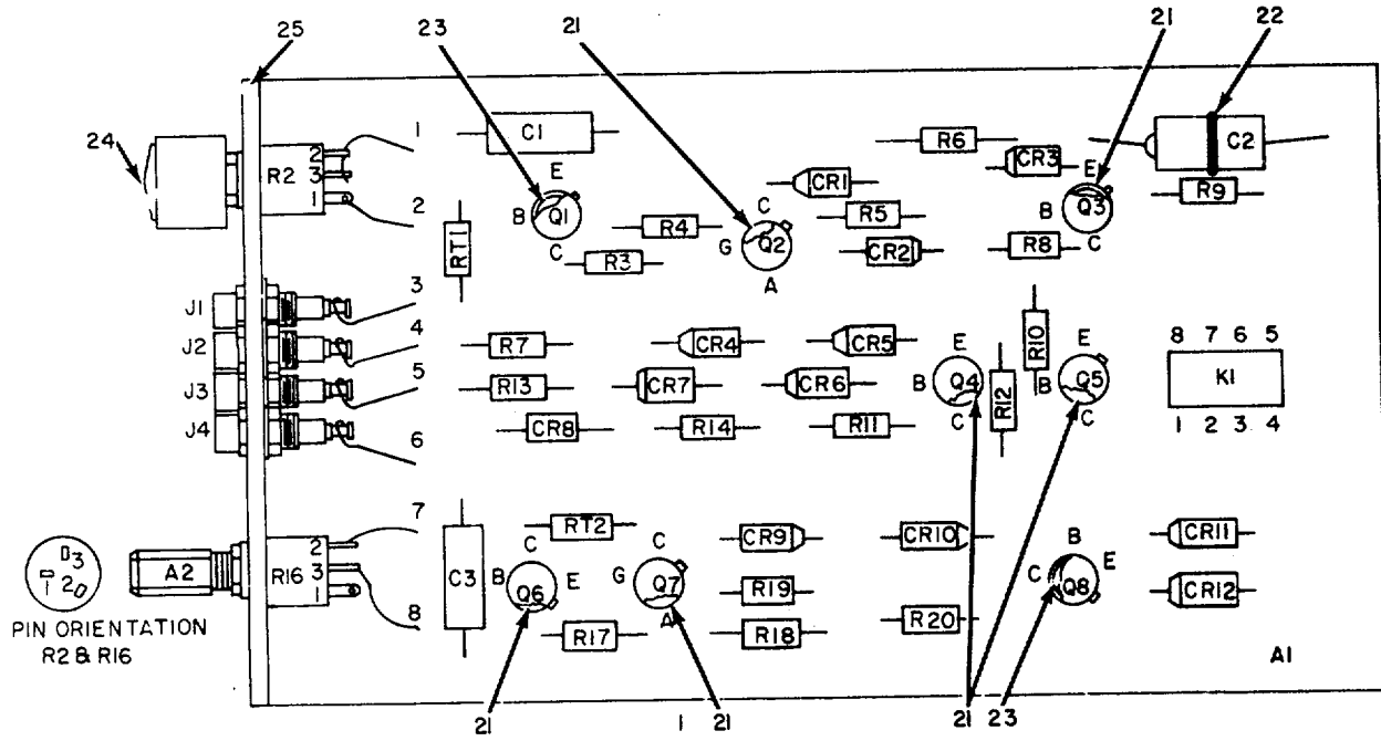
Figure 40. Control, Alarm, Low Radio Frequency-Mismatch 3A4.
