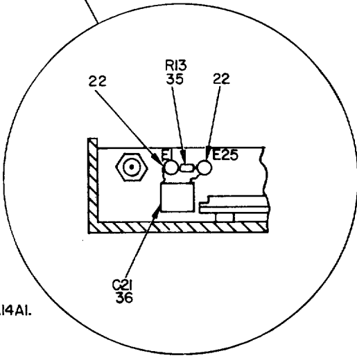
Figure 23. Oscillator, Radio Frequency 1A14A1.
